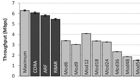
Fig. 6. Average throughput for each algorithm and fixed data rates in Scenario 1
