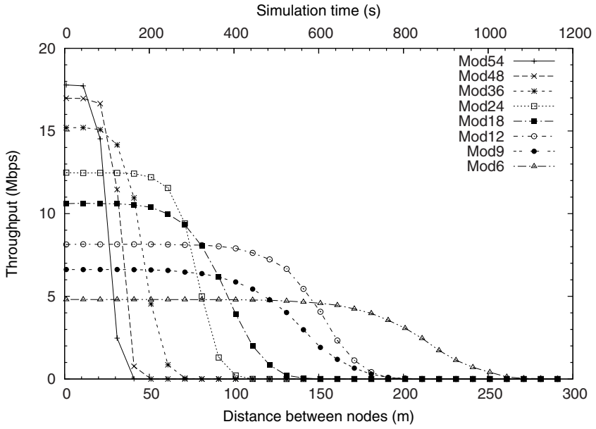
Fig. 4. Throughput over distance for 802.11g fixed data rates
