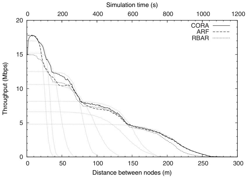
Fig. 5. Throughput over distance for each rate adaptation algorithm
